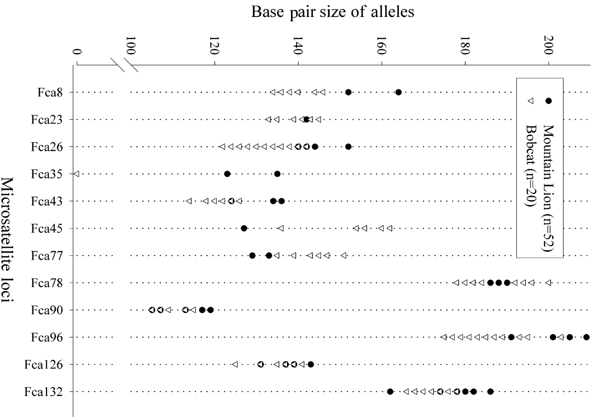
Fig. 2 Allele base pair sizes for 12 microsatellite loci examined in mountain lions (grouped subset, n = 52 ) and bobcats ( n = 20 ).
